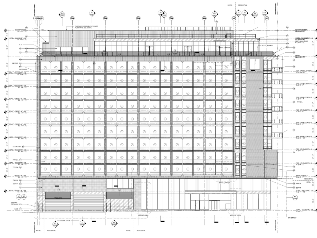
1. North Elevation
